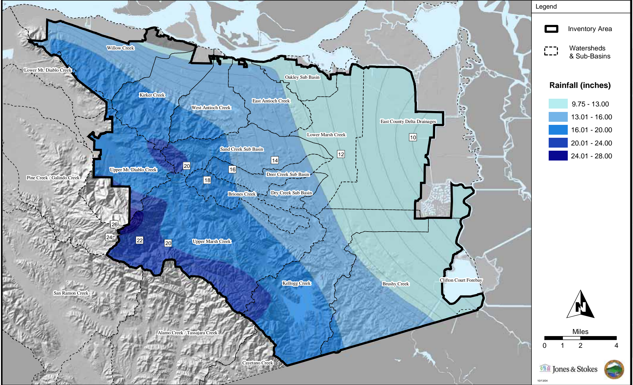
Figure 3-3 Regional Precipitation
